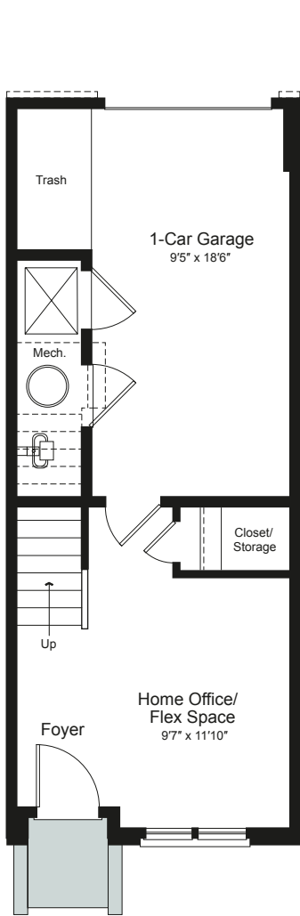
ENTRY LEVEL w/ Garage
