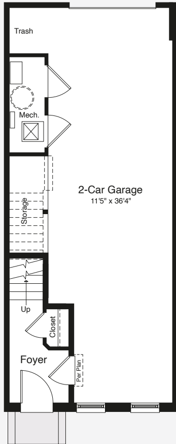
ENTRY LEVEL
