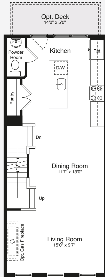
MAIN LEVEL
