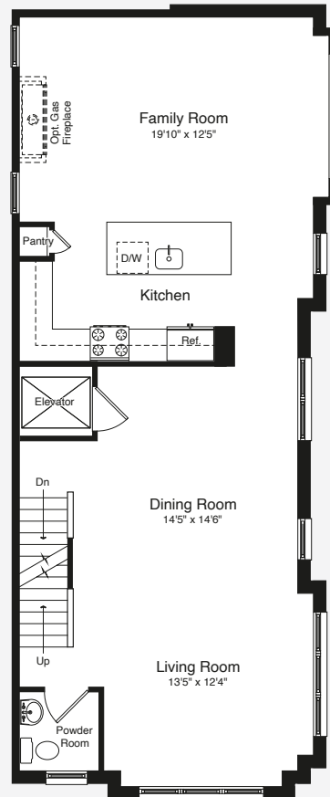
MAIN LEVEL
