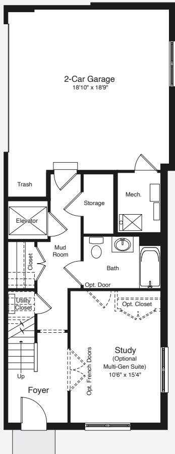
ENTRY LEVEL
