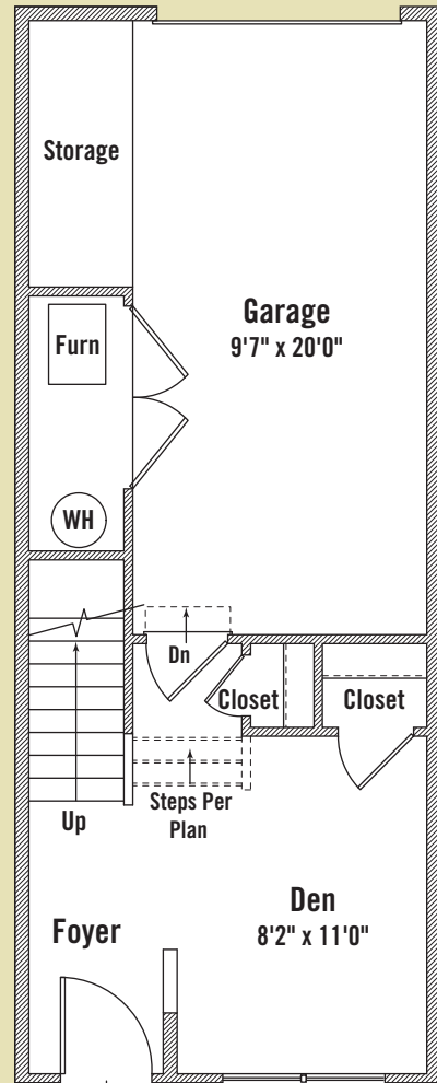
ENTRY LEVEL (OPT. 2 CAR GARAGE AVAIL.)
